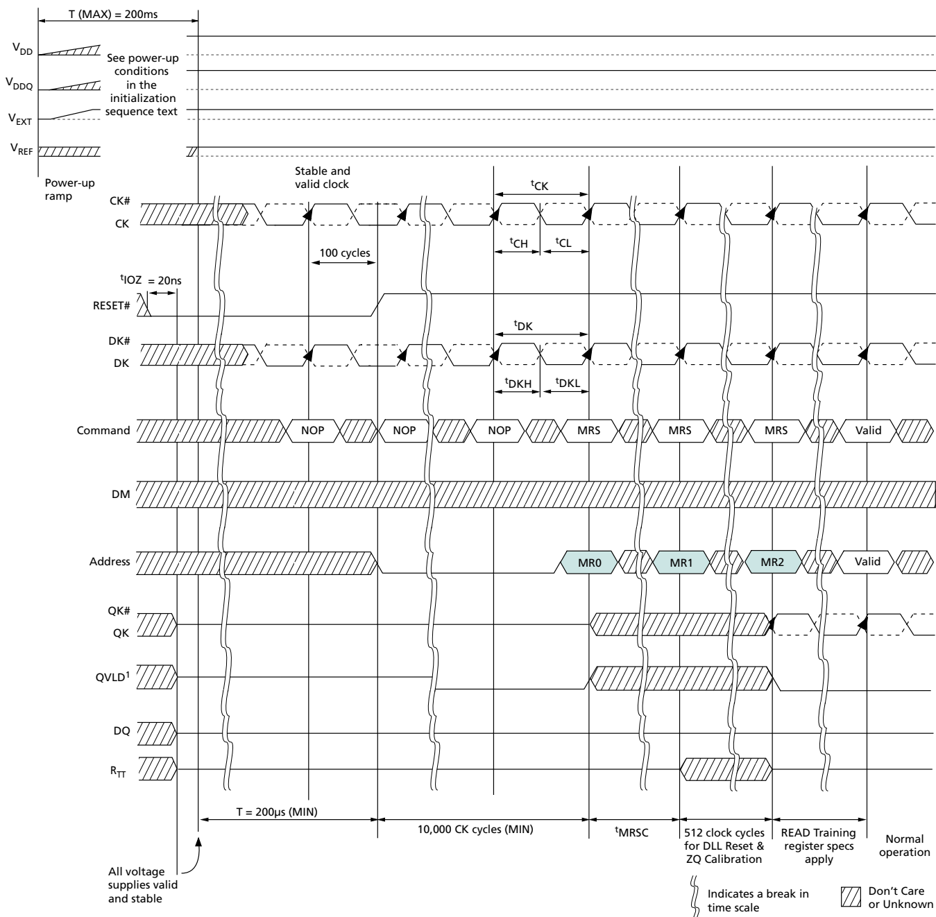
Figure 41: Power-Up/Initialization Sequence
