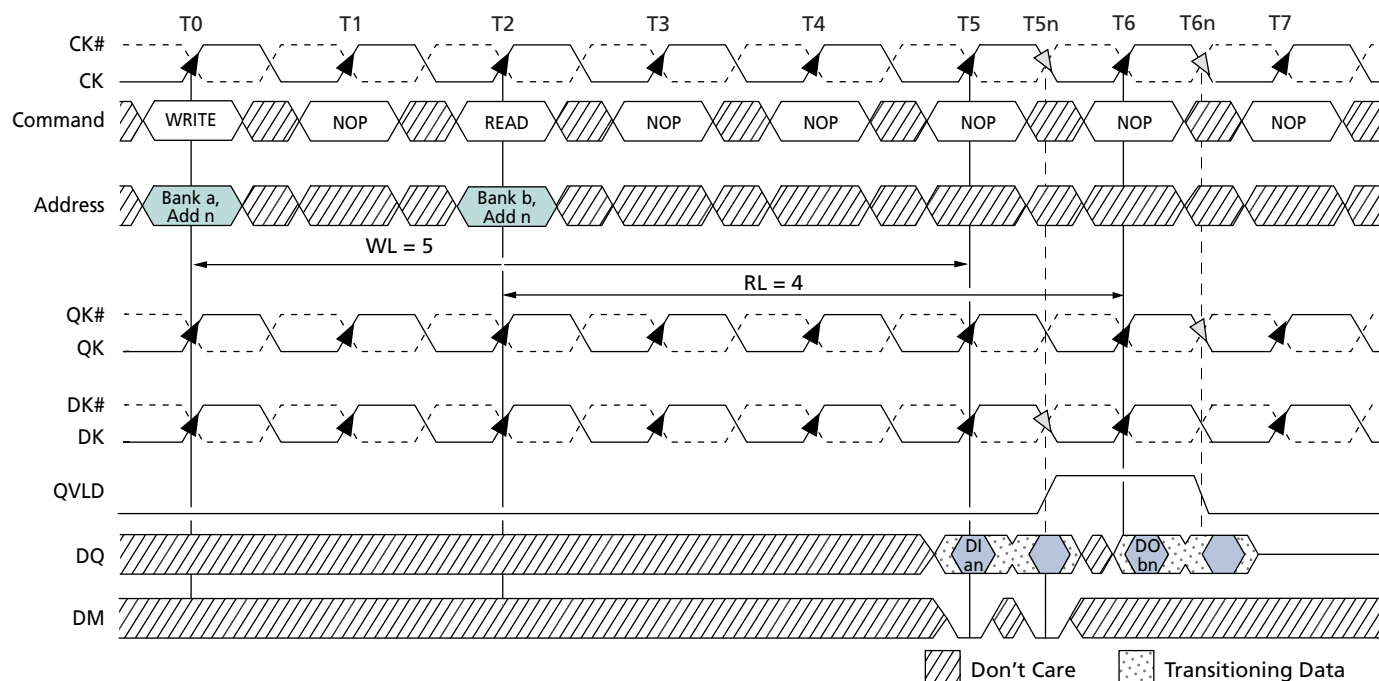
Figure 44: WRITE-to-READ
