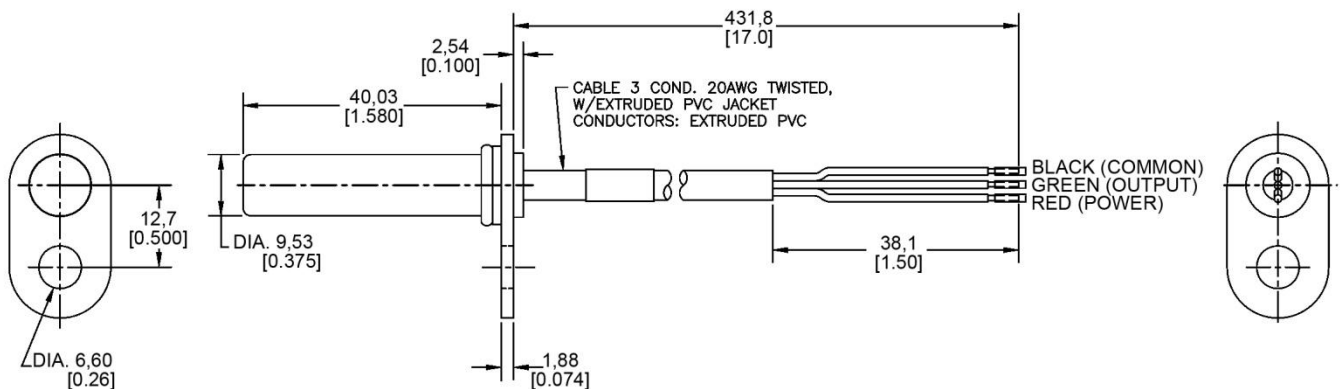
Figure 1. Mounting Dimensions and General Mounting Geometry (For reference only: mm [in.] )
