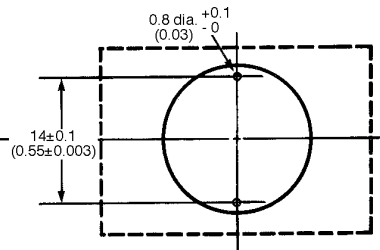
Mounting hole (bottom view)
