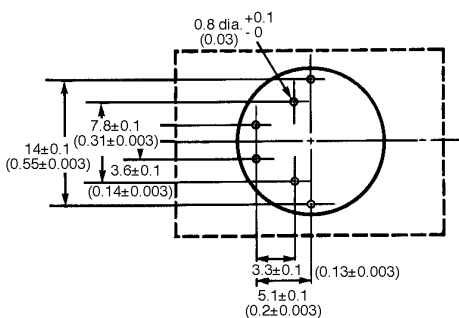
Mounting hole (bottom view)
