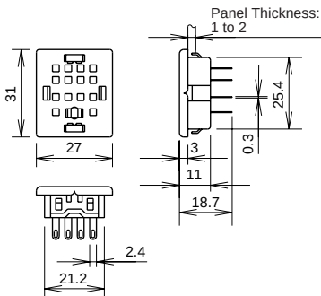
Terminal Arrangement
