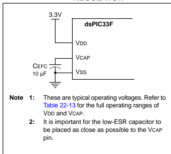
FIGURE 19-1: CONNECTIONS FOR THE ON-CHIP VOLTAGE REGULATOR (1)
