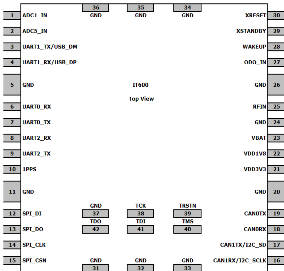
Figure 3 Pin-out
