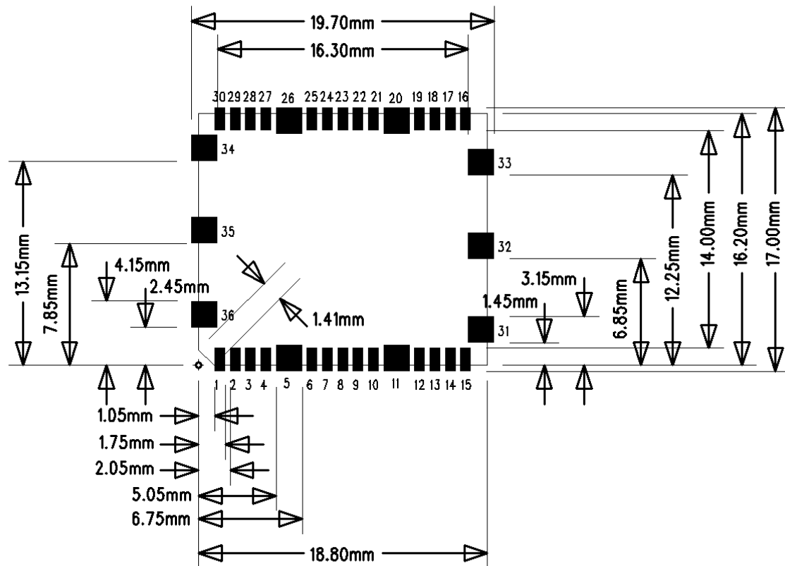
Figure 7 Suggested pad layout and occupied area, Top view. Suggested paste mask openings equal pad layout
