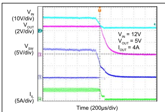
FIGURE 2-27: Turn-Off.
