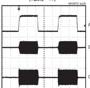
50% BRIGHTNESS DWPM WAVEFORM ( V_{CNTL} = 1V )
