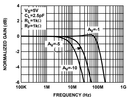
FIGURE 4. SMALL SIGNAL FREQUENCY RESPONSE FOR VARIOUS INVERTING GAINS
