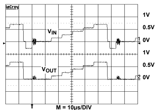
FIGURE 33. VIDEO SIGNAL
