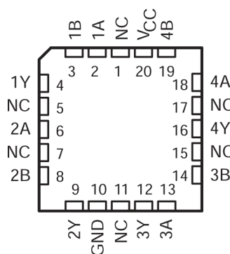
Figure 3-3. SN54ACT86 FK Package (Top View)
