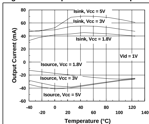
Figure 23. Output current vs. temperature
