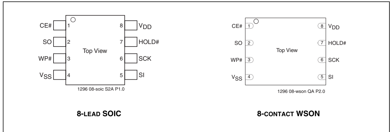
FIGURE 1: PIN ASSIGNMENTS
