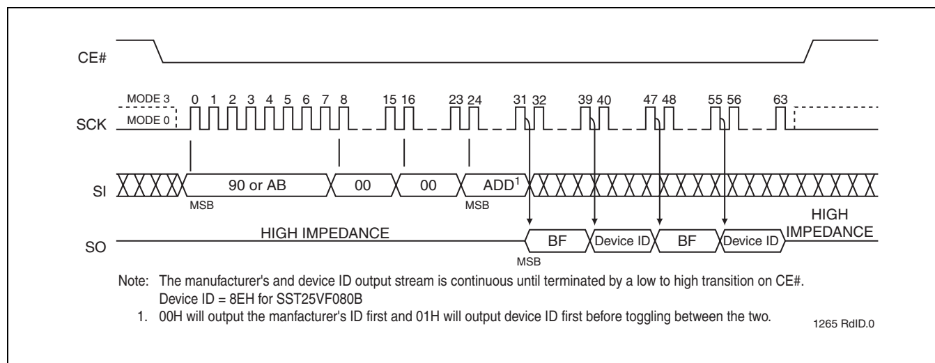
FIGURE 20: READ-ID SEQUENCE
