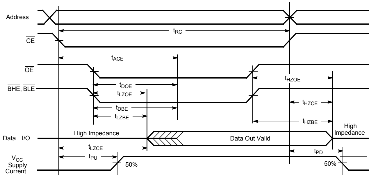
Figure 4. Read Cycle No. 2 ( \overline{OE} Controlled) [16, 17]
