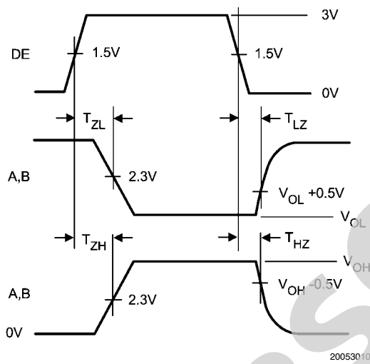
FIGURE 8. Driver Enable / Disable Time
