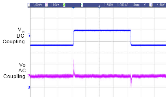
9. Line Transient Response
