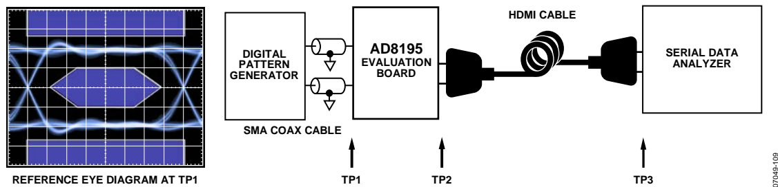
Figure 13. Test Circuit Diagram for Tx Eye Diagrams
