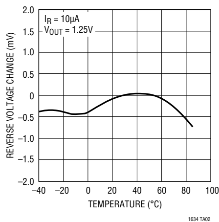
Temperature Drift
