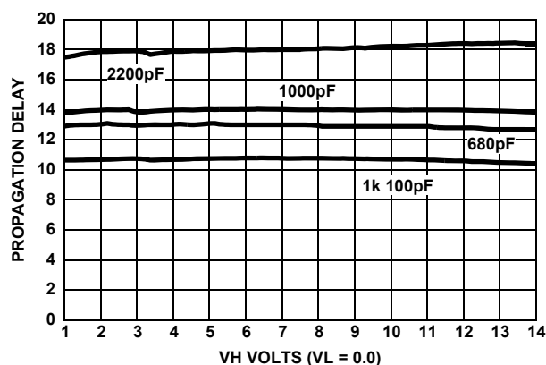
FIGURE 12. PROPAGATION DELAY vs VH RAIL, VARIOUS LOADS
