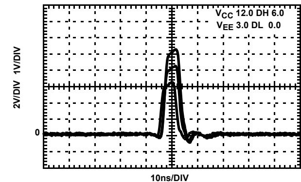
FIGURE 20. MINIMUM PULSE WIDTH VH 6/8/10V
