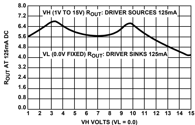
FIGURE 11. R_{OUT} vs VH RAIL
