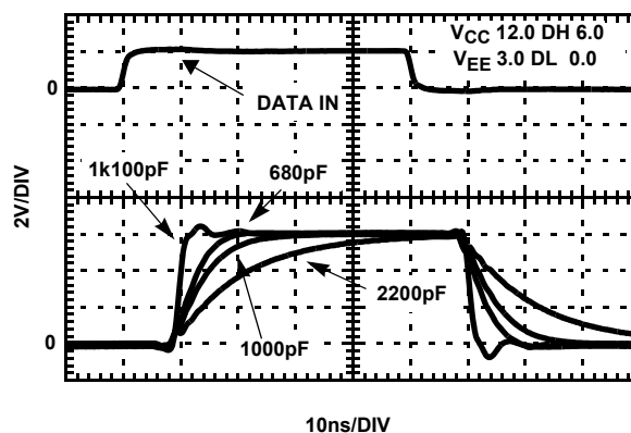
FIGURE 8. DRIVER WAVEFORMS UNDER VARIOUS LOADS
