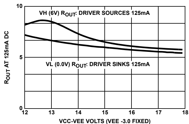
FIGURE 10. R_{OUT} vs DEVICE VOLTAGE
