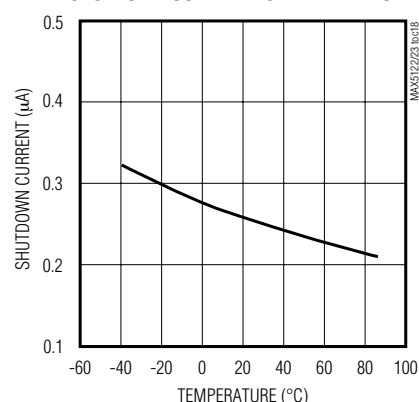
MAX5123 SHUTDOWN CURRENT vs. TEMPERATURE
