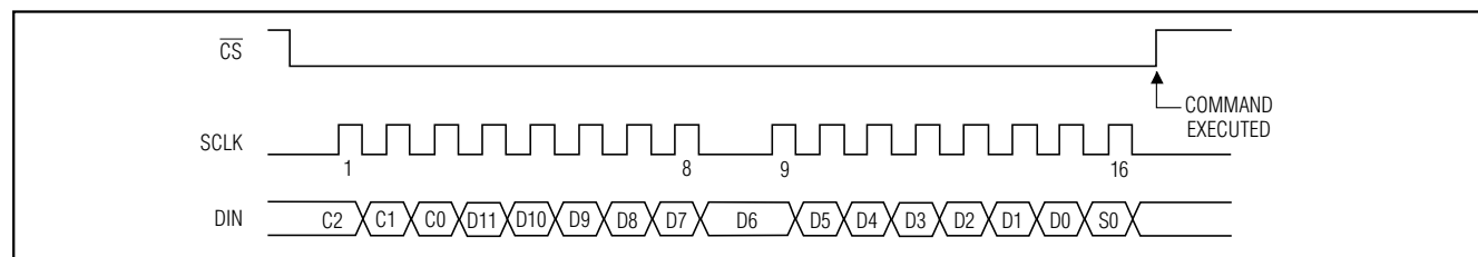
Figure 6. Serial-Interface Timing
