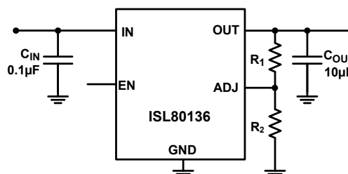
FIGURE 14. SETTING OUTPUT VOLTAGE
