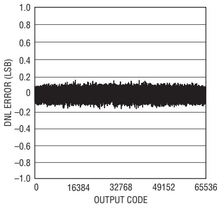
LTC2190: Differential Nonlinearity (DNL)
