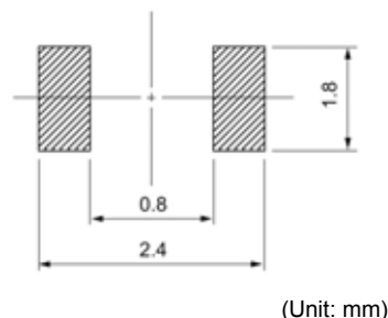
Recommended patterns 推荐焊盘尺寸
