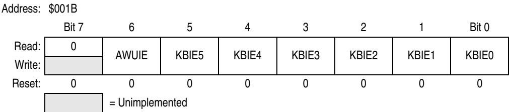
Figure 9-4. Keyboard Interrupt Enable Register (KBIER)
