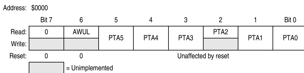
Figure 4-2. Port A Data Register (PTA)
