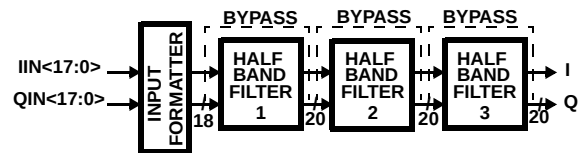
FIGURE 2. INPUT FORMATTER AND INTERPOLATOR BLOCK DIAGRAM
