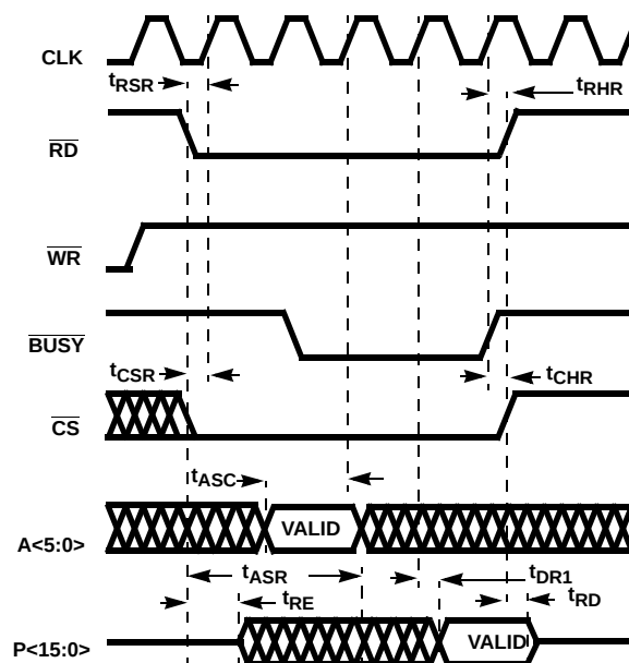
FIGURE 22. MICROPROCESSOR READ TIMING
