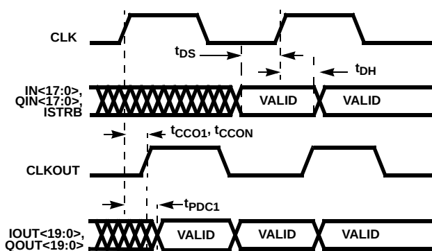
FIGURE 17. INPUT/OUTPUT TIMING
