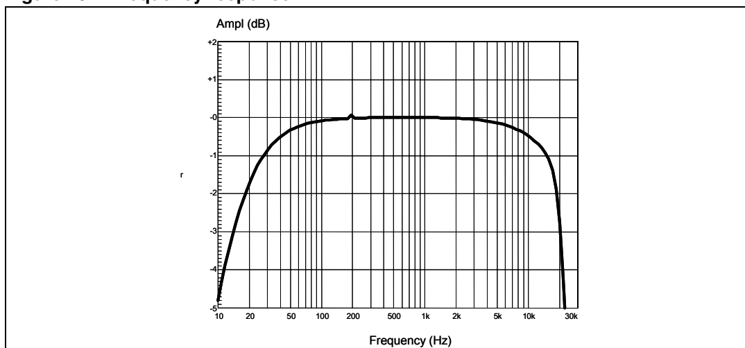
Figure 17. FFT (0 dB)
