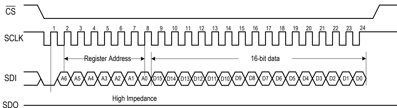
Figure-7 Write Sequence in Four-Wire Mode
