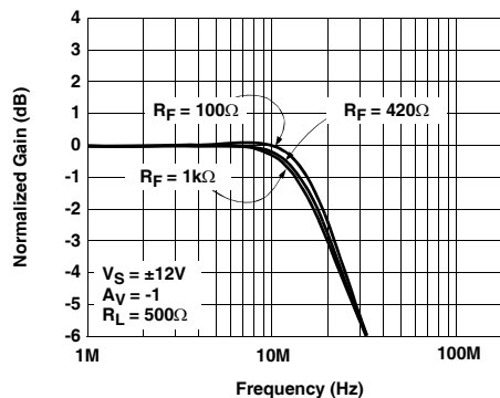
Inverting Frequency Response (Gain)
