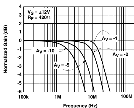
Inverting Frequency Response (Gain)
