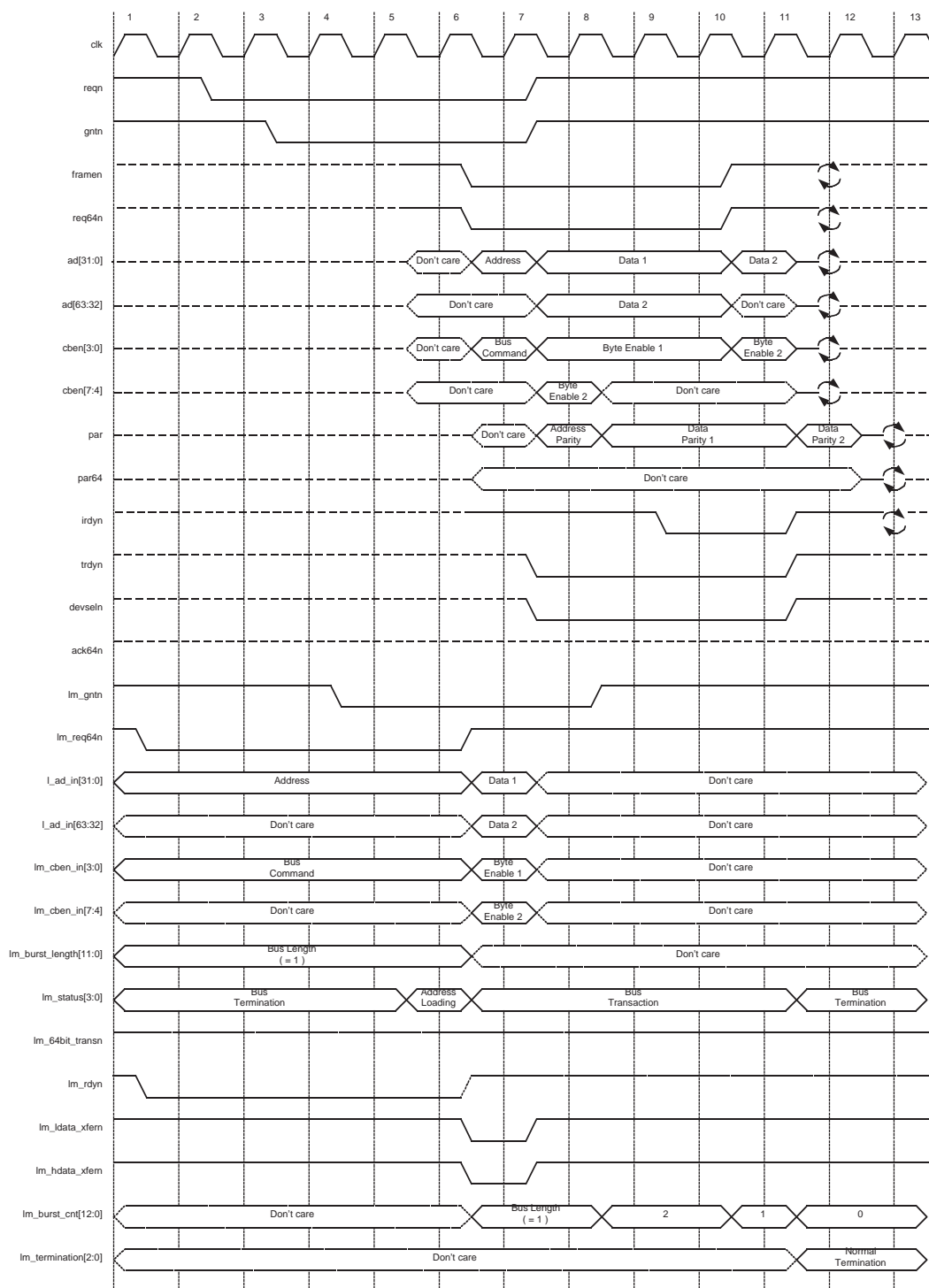
Figure 2-12. 32-bit Master Single Write Transaction with a 64-bit Local Interface
