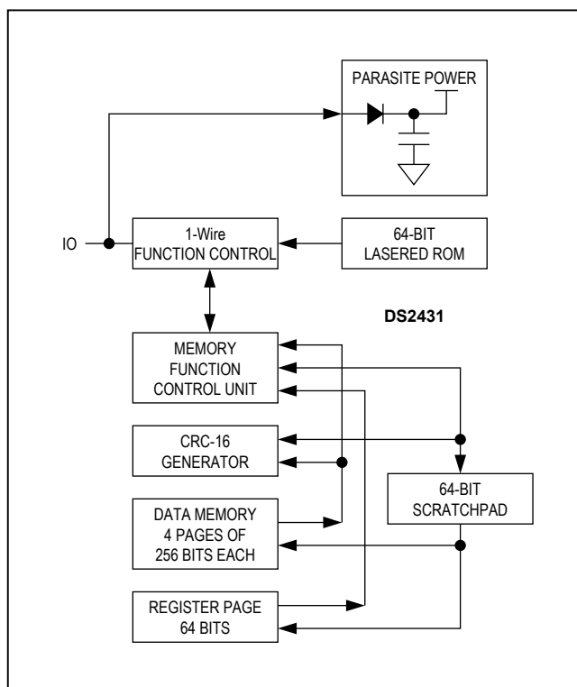
Figure 1. Block Diagram
