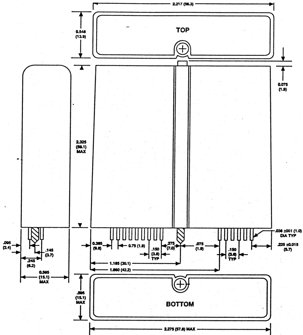
Figure 5. Outline Dimensions
