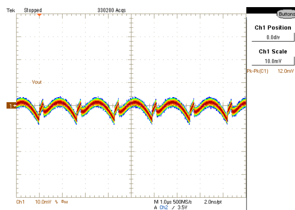
Figure 36: Output Voltage Ripple at full load CH1:Vout
