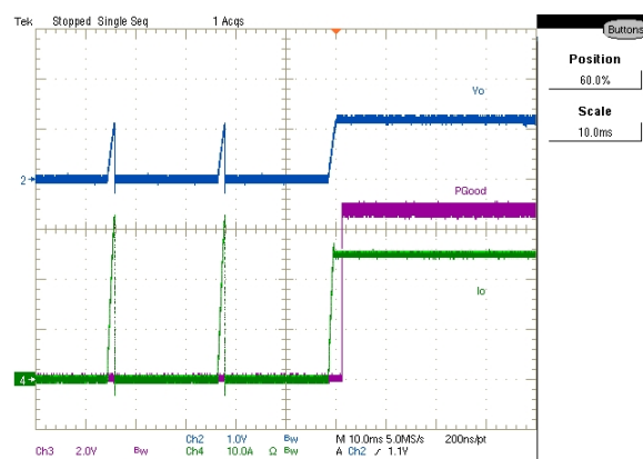
Figure 34: Recovery from Hiccup CH2:Vout, CH3:PGood, CH4:Iout
