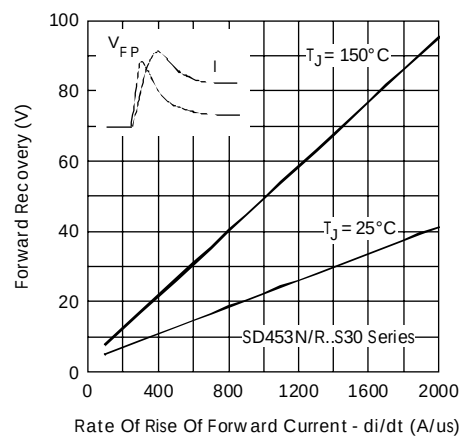
Fig. 17 - Typical Forward Recovery Characteristics
