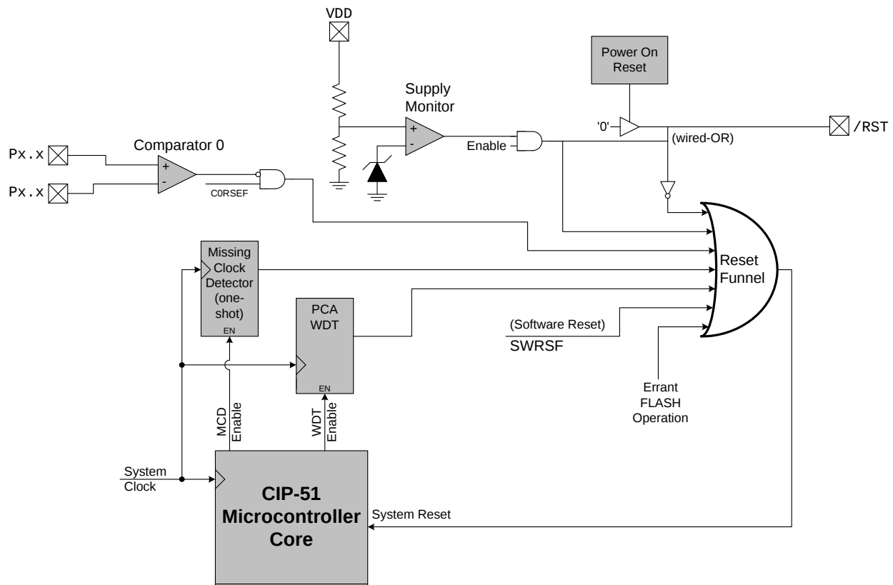
Figure 10.1. Reset Sources
