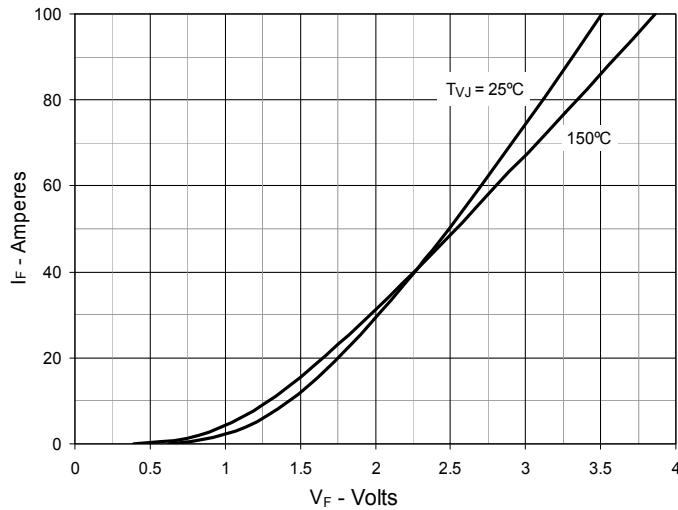
Fig. 22. Forward Current vs. Forward Voltage
