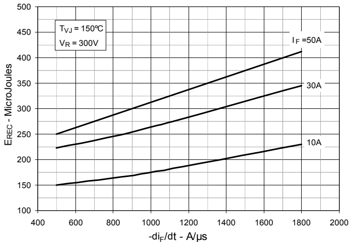
Fig. 26. Recovery Energy E_{REC} vs. -di_F/dt
