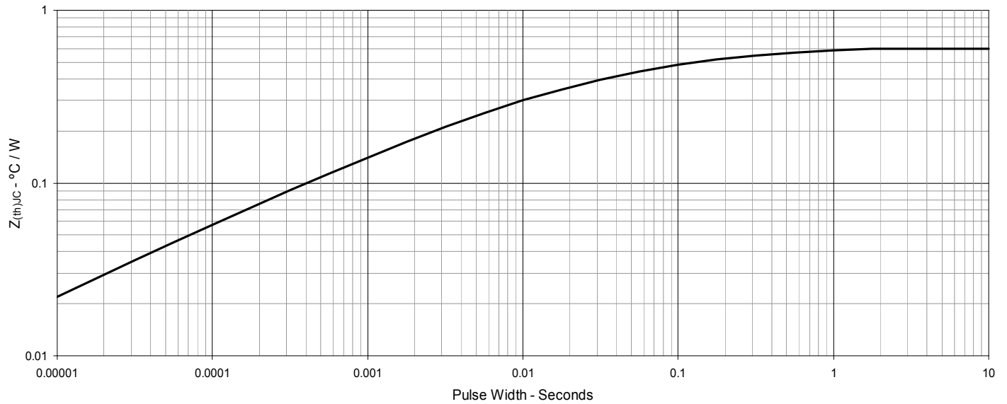
Fig. 28. Maximum Transient Thermal Impedance (Diode)
