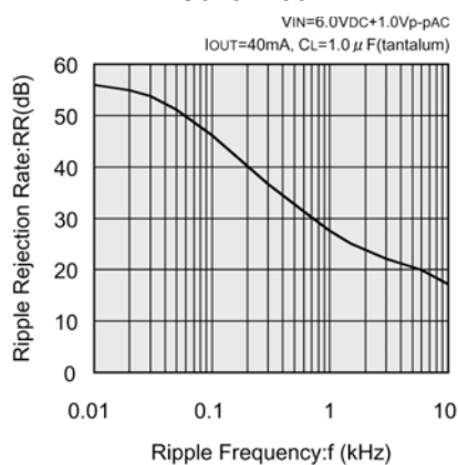
XC6201P502
