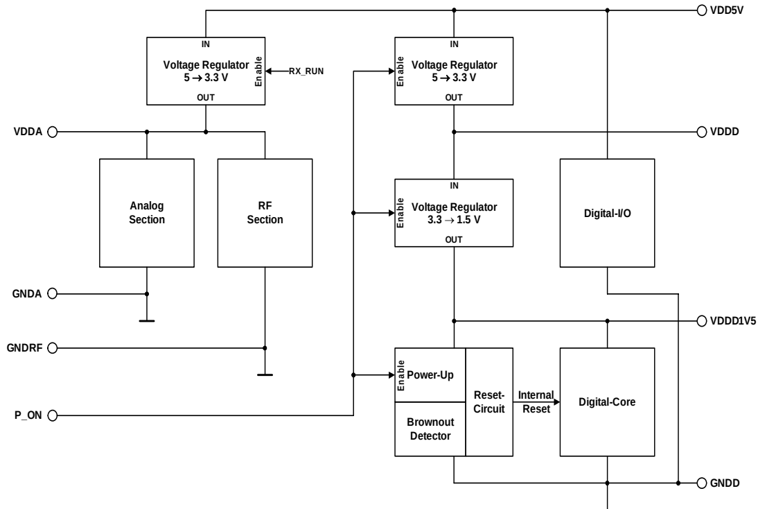
Figure 18 Power Supply
