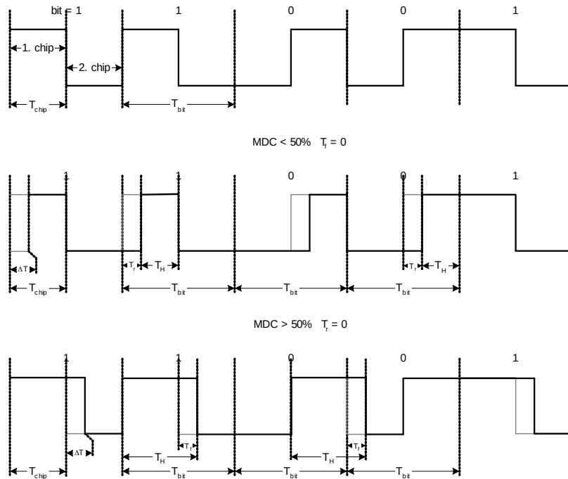
Figure 50 Definition C: Edge delay definition
