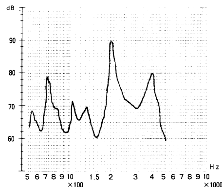
Fig.5 Frequency response with resonator (Design II)
