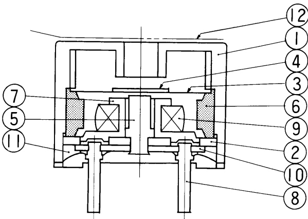
Fig.1 Construction view of type QMX
