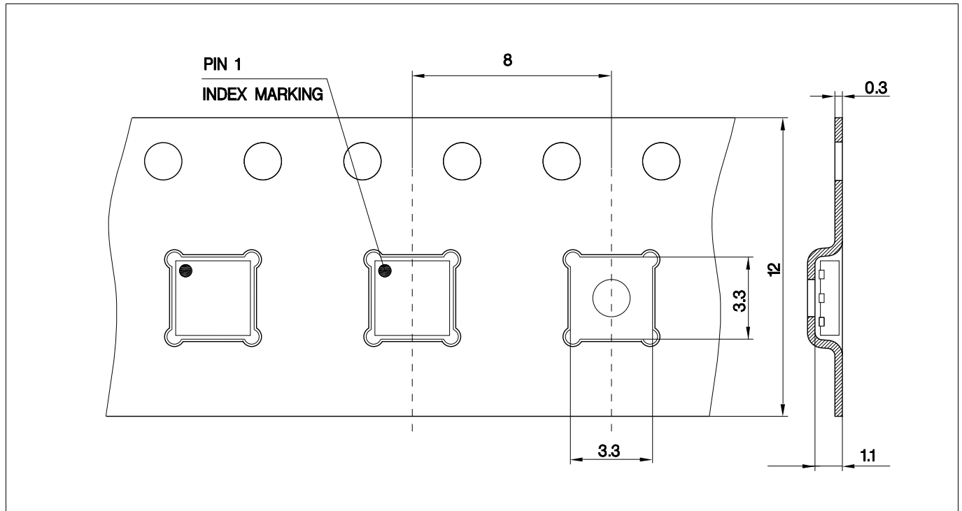
Figure 25 PG-WSO6-1 Packaging Dimensions
