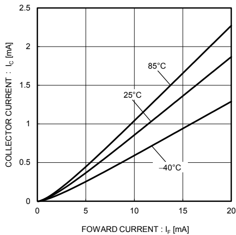
Fig.9 Output Characteristics
