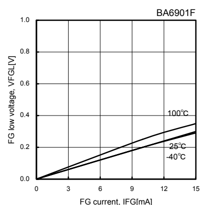
Fig.27 FG Output L voltage
