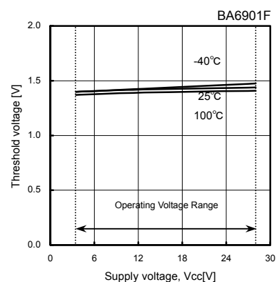
Fig.30 PWM input threshold voltage
