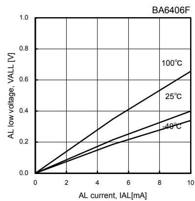
Fig.18 AL output L voltage
