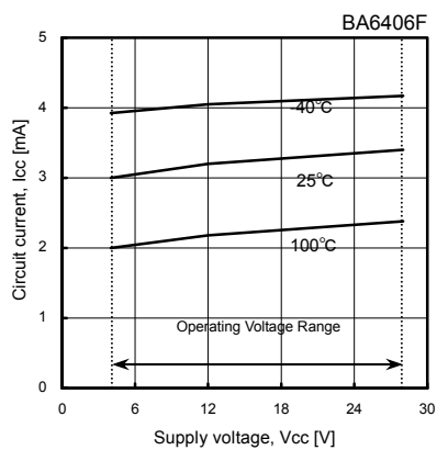
Fig.16 Circuit current
