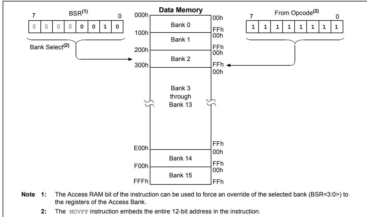
FIGURE 6-9: USE OF THE BANK SELECT REGISTER (DIRECT ADDRESSING)
