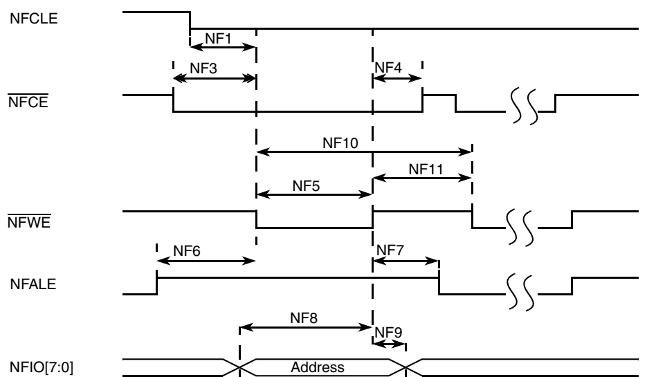
Figure 12. Address Latch Cycle Timing Diagram
