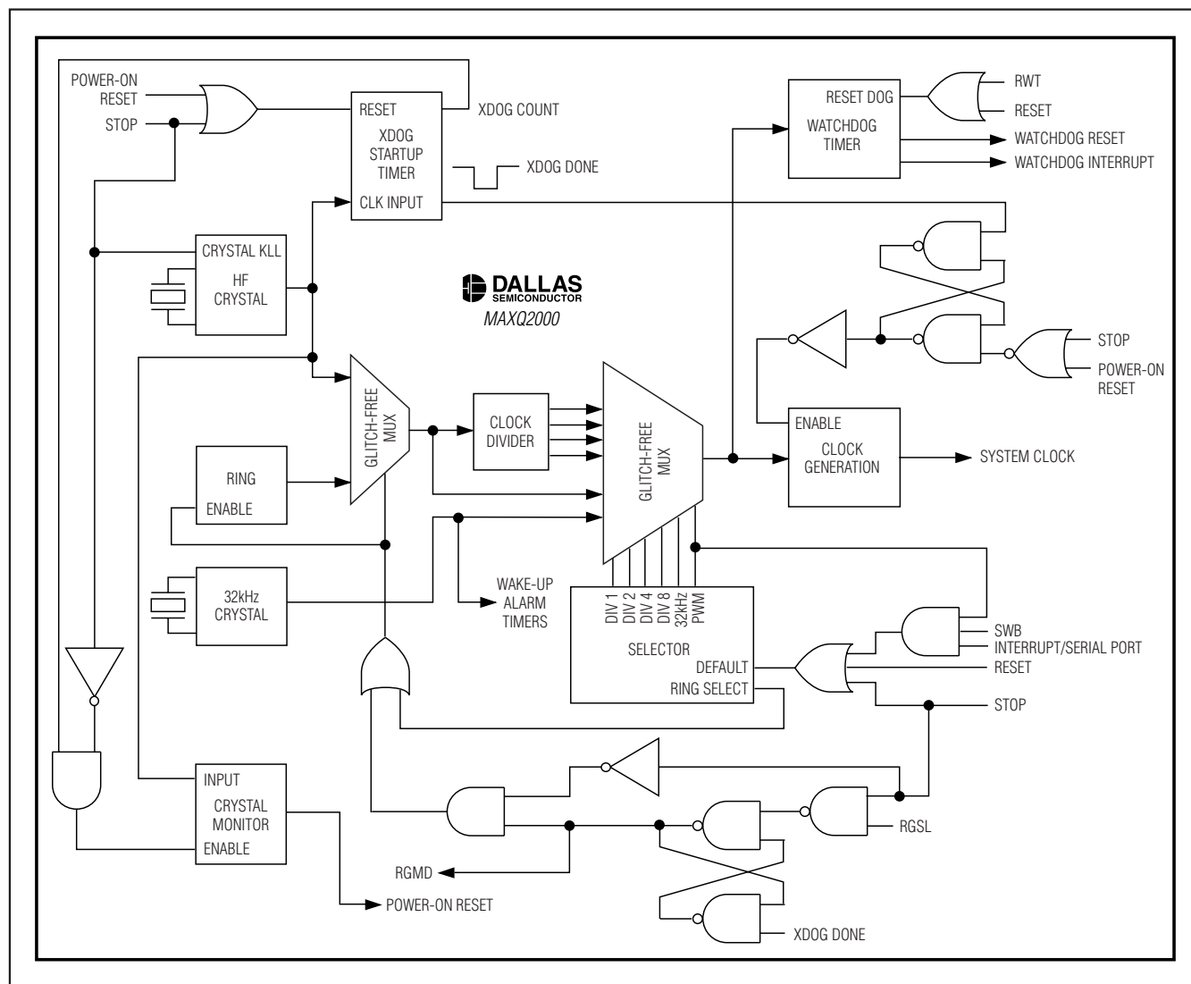
Figure 2. Clock Sources
