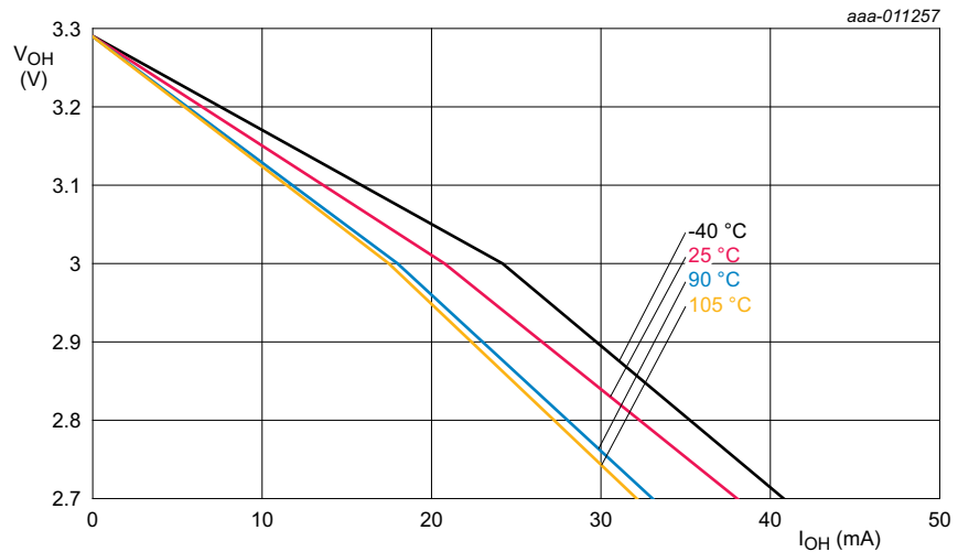
Fig 25. High-drive output: Typical HIGH-level output voltage V_{OH} versus HIGH-level output current I_{OH}
