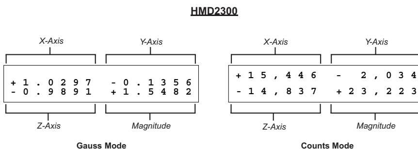
Figure 1. Sample output when connected to an HMR2300
