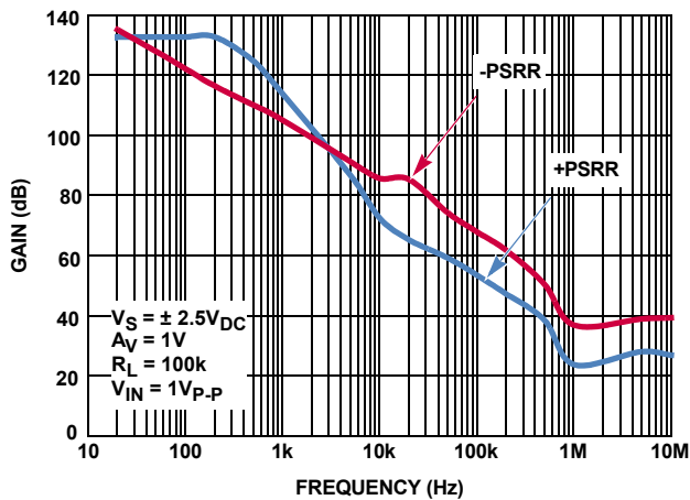
FIGURE 36. PSRR vs FREQUENCY, V_S = 5V
