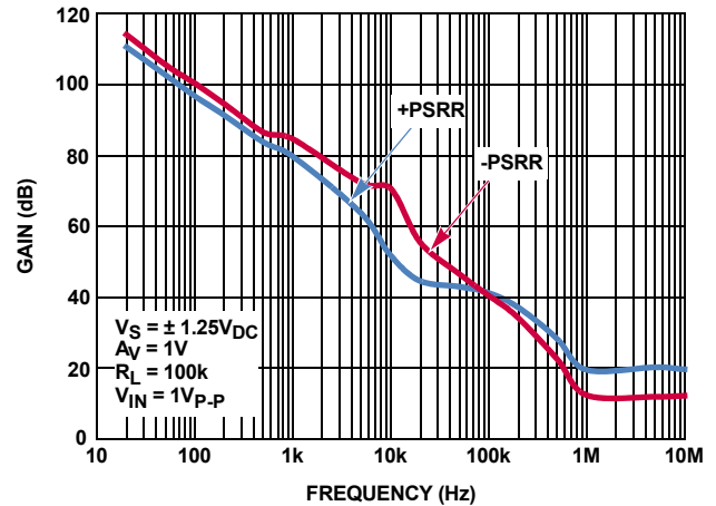
FIGURE 37. PSRR vs FREQUENCY, V_S = 2.5V
