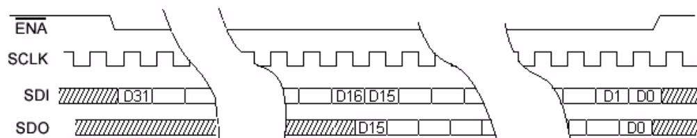
Serial Timing Diagram (32 bit)
