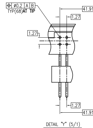
DETAIL "Y" (5/1)
