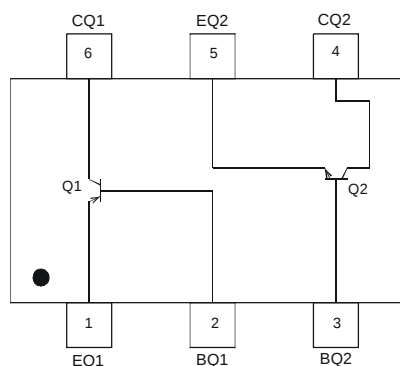
Schematic and Pin Configuration
