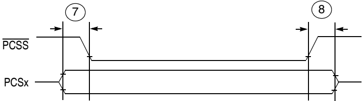
Figure 26. DSPI PCS Strobe ( \overline{\text{PCSS}} ) Timing
